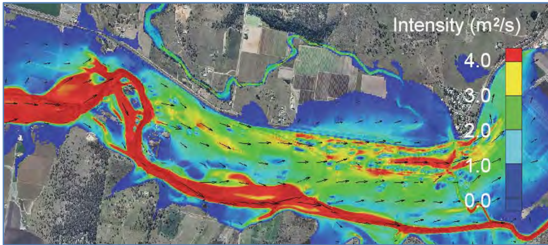
Figure 5.26: Image of modelled water levels at 4:35 pm on 10 January 2011 Source: Exhibit 304, John Macintosh, Most likely scenario animation
