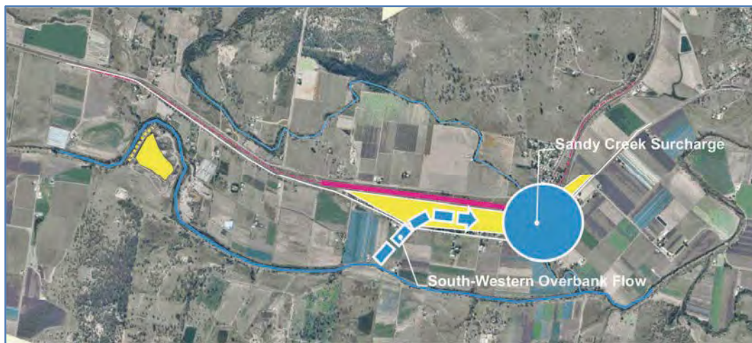
Figure C12: Simplified flooding locality, south-western overbank inundation. Source: Exhibit 144, Dr John Macintosh, Report to Grantham Floods Commission of Inquiry – Expert Hydrology Report 10 January 2011 – Circumstances and Contributing Factors , 11 August 2015 [p21: Figure 1.3(b)]
