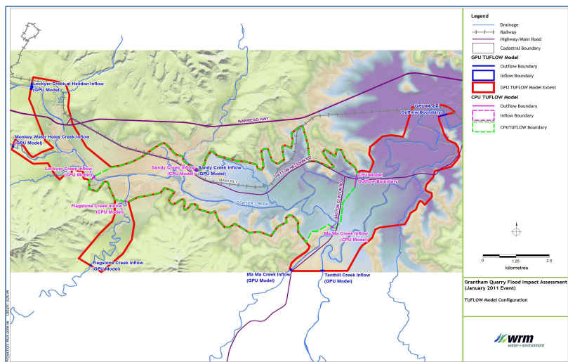
Figure C40: Boundaries of the GPU and CPU models.
