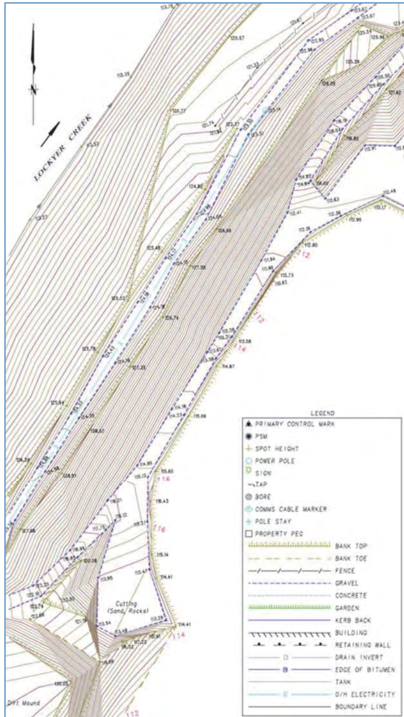
Figure A14: Detail from survey plan of Grantham quarry prepared for Wagners in 2008 Source: Exhibit 131, Mr David Starr, Grantham quarry – geotechnical investigations and expert opinion on formation of earthworks , Revised 28 August 2015 [p39: Plate 29]
