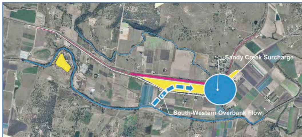
Figure 5.6: Diagram of second stage of flooding Grantham
