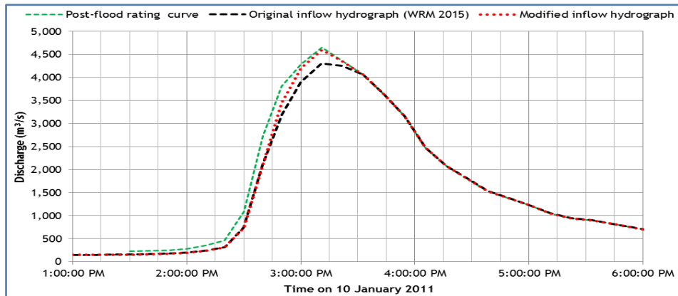
Figure C41: Inflow hydrograph.
